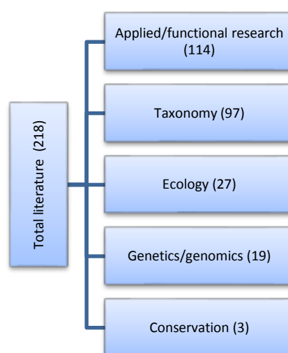
Figure 8.7 Number of publications on soil bacteria in different subject focus in IHR.
