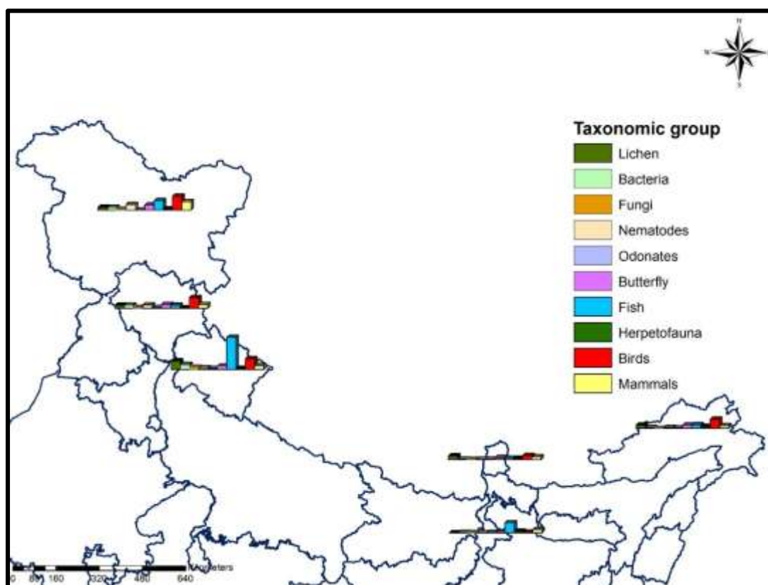
Figure 1.2 State-wise distribution of Literature on the fauna and micro flora of the Indian Himalayan Region
