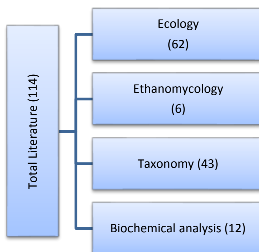
Figure 8.5 Publication on Fungi by subject focus in IHR.
