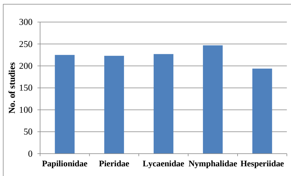
Figure 6.3 Distribution of scientific literature among different families
