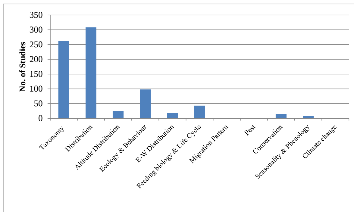
Figure 6.4 Number of publications on butterflies of the Indian Himalayan Region in different subject categories
