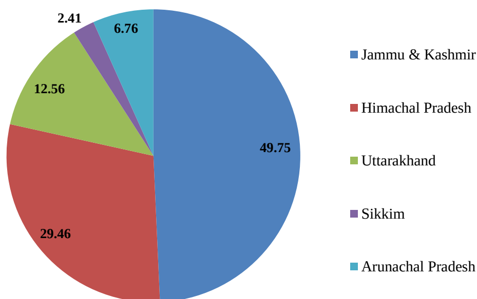
Figure 7.1 State wise distribution of publications
