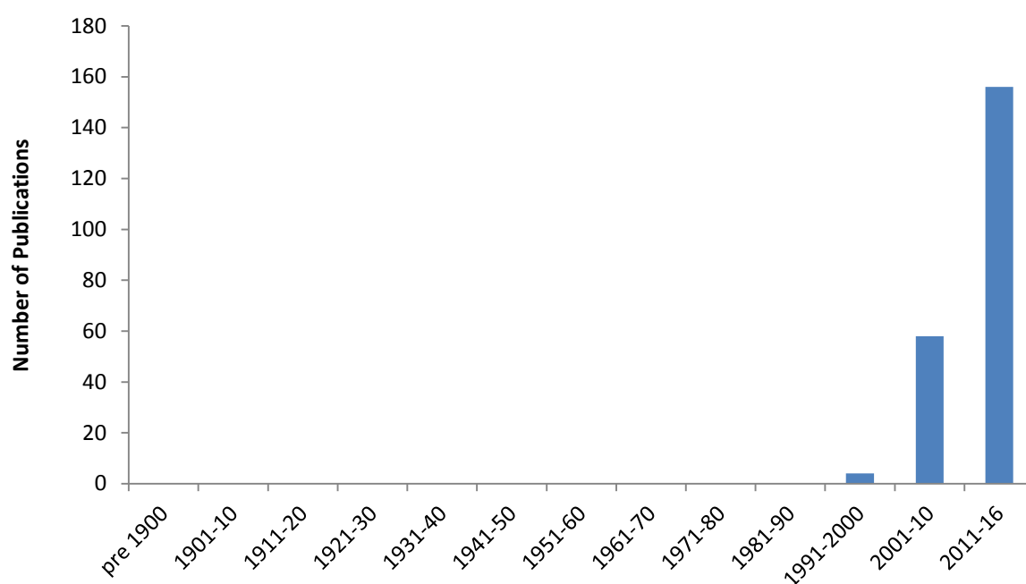
Figure 8.6 Temporal pattern of publication on soil bacteria of Indian Himalayan Region
