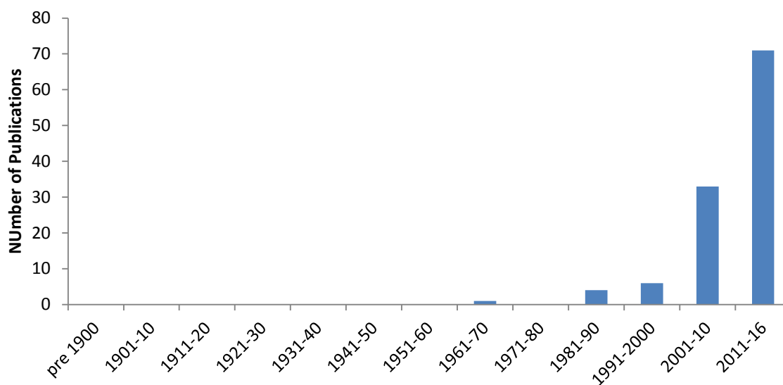
Figure 8.4 Temporal pattern of publication on soil fungi of Indian Himalayan Region
