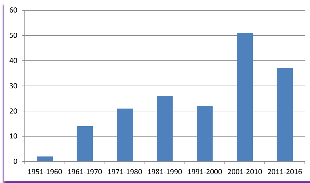
Figure 7.2 Temporal pattern of publications on nematodes of Indian Himalayan Region
