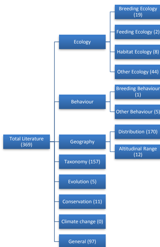
Figure 4.4 Number of publications on the herpetofauna of the Indian Himalayan Region in different subject categories
