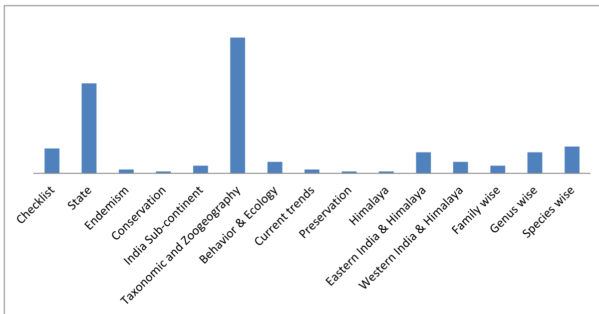
Figure 6.6 Comprehensive classifications of publication on odonates of the Indian Himalayan Region
